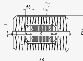
Vista Frontal Front View / Vista Frontal
