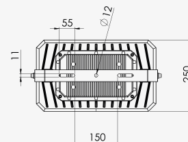
Vista Frontal Front View / Vista Frontal
