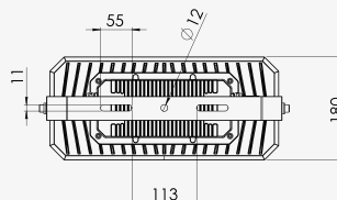
Vista Frontal Front View / Vista Frontal
