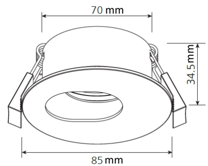
Oval Hole Trim Ø80
