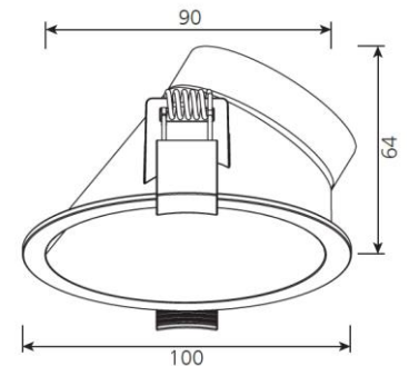
Asymmetrical Trim Ø95
