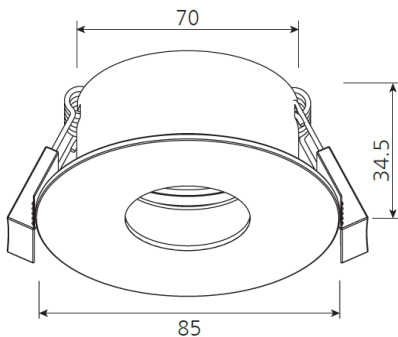
Circular Hole Trim Ø80
