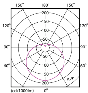
Light Distribution Diagram - EcoHome LEDBulb 8W E27 6500KHV 1PF/20AR
